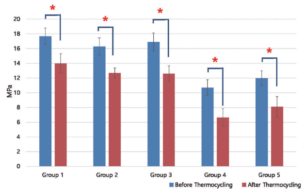
Fig. 5. Mean and standard deviation of shear bond strength of zirconia discs contaminated with saliva after various cleaning methods and control group. Significant at \rho < 0.05 level (*).
