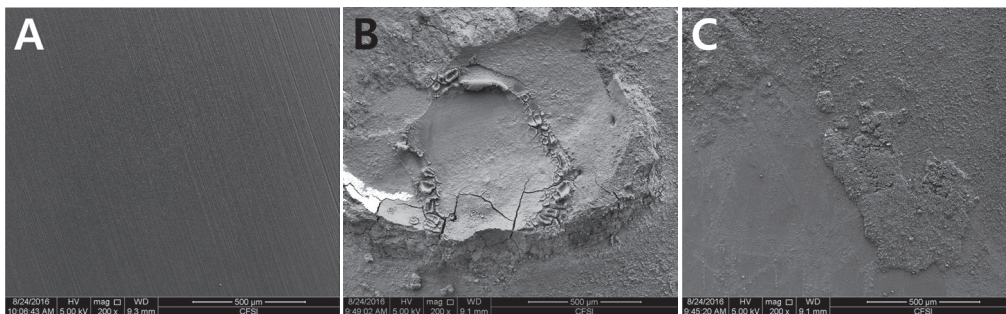
Fig. 4. Representative scanning electron microscope image of fracture mode on zirconia discs (200). (A) Adhesive failure, (B) cohesive failure, (C) mixed failure.
