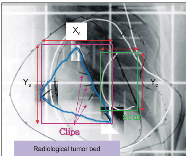
Fig. 2. Simulation film showing lumpectomy scar and surgical clips. (the enclosed area is the radiologically determined tumor bed, one clip is on the clinically defined field border). X_s : width of surgical field, Y_s : height of clip-based surgical field, X_c : width of clinical field, Y_c : height of scar-based clinical field.
